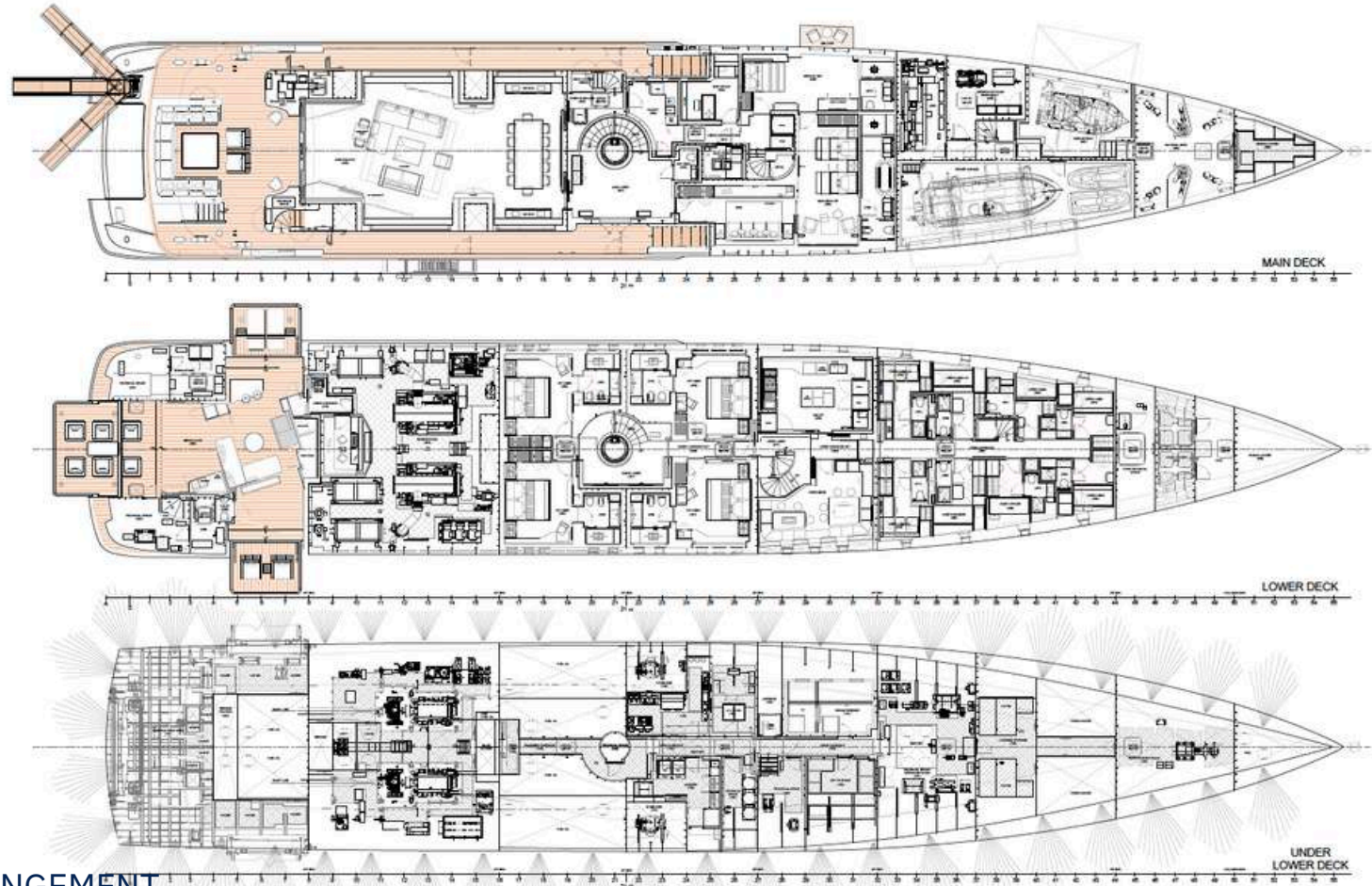
GENERAL ARRANGEMENT
