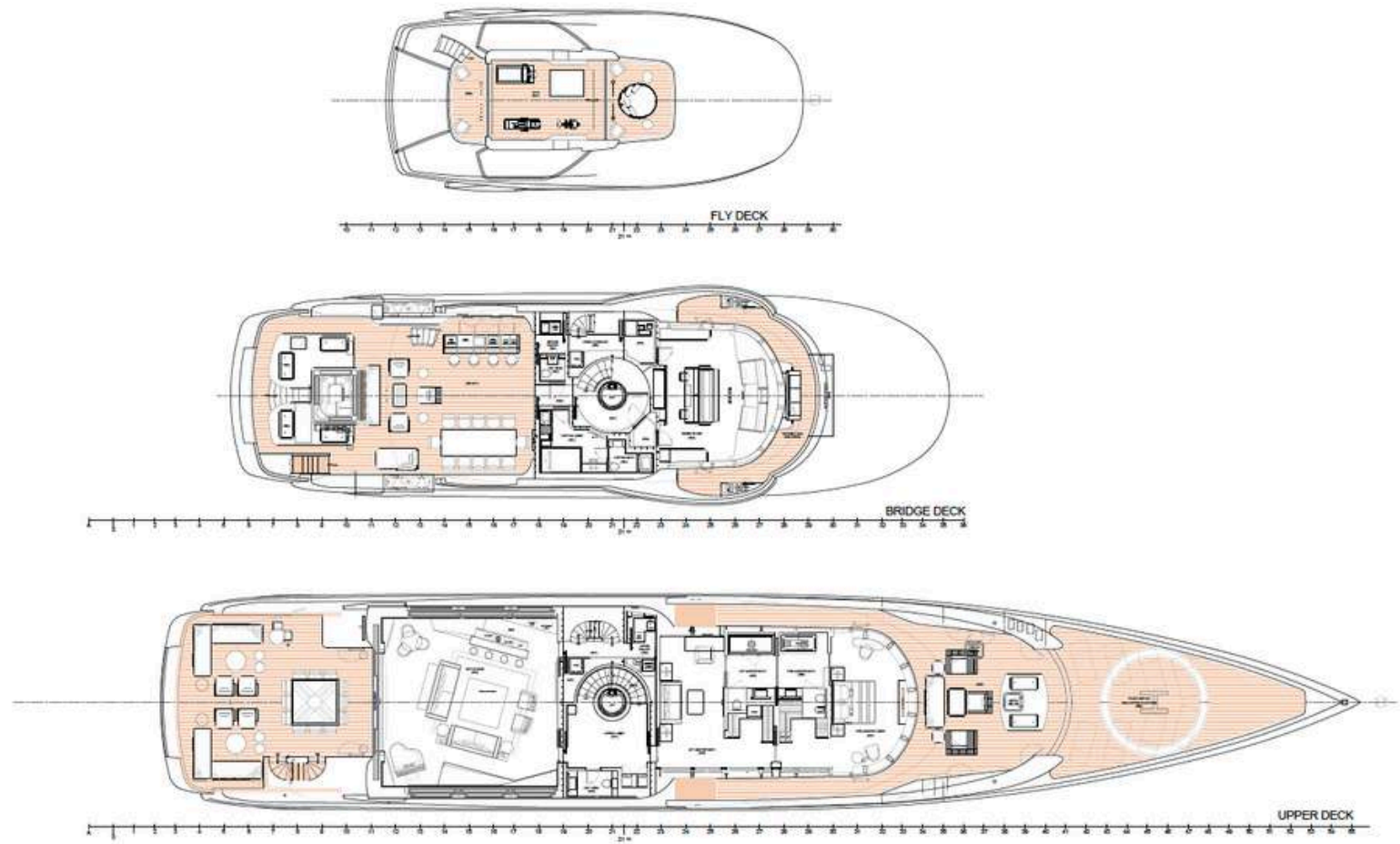
GENERAL ARRANGEMENT
